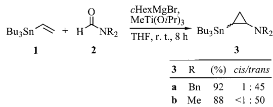
Scheme 1. Synthesis of 2-(trialkylstannyl)- N,N -dialkylcyclopropylamines 3
