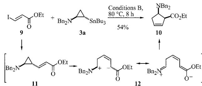
Scheme 5. Cross coupling of N,N -dibenzyl-2-(tributylstannyl)cyclopropylamine ( 3a ) with ethyl trans -3-iodoacrylate ( 9 ) and subsequent rearrangement to yield ethyl cis -5-(dibenzylamino)cyclopent-2-enecarboxylate ( 10 )
