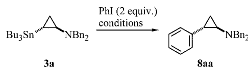
Scheme 3. Cross coupling of cyclopropylstannane 3a with phenyl iodide; for details see Table 1
