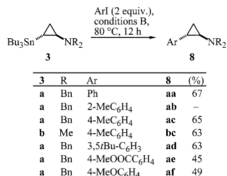
Scheme 4. Palladium-catalyzed cross-couplings of 2-(trialkylstannyl)- N,N -dialkylcyclopropylamines 3 with various aryl iodides under optimized conditions B (see Table 1)
